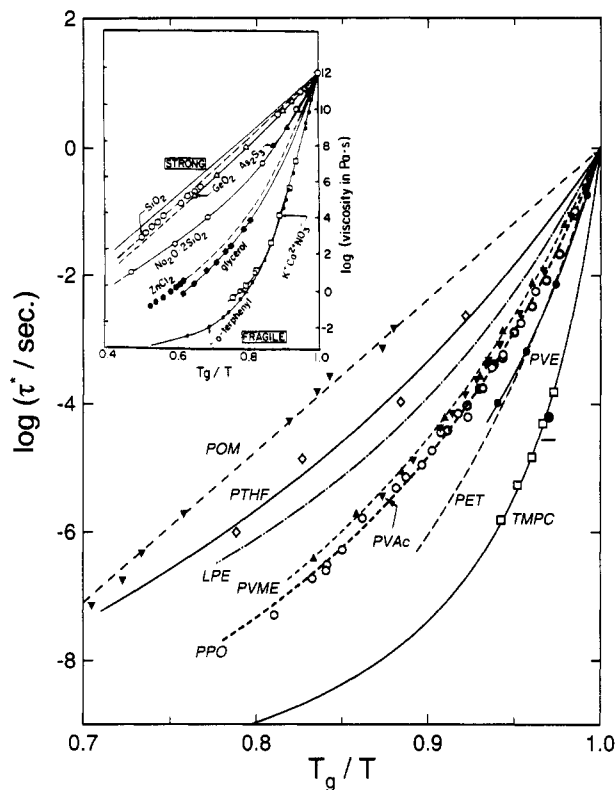
Figure 6. Cooperativity plots for a variety of polymers, representing the extremes from strong intermolecular coupling in tetramethyl polycarbonate to the almost Arrhenius behavior of poly(oxyethylene). The inset shows the original T_g -scaled plots of shear viscosity of Angell 43 for small molecular and network glass-forming liquids.
